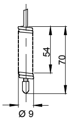
Sensor type A Vapour charge 2 m capillary with bulb
