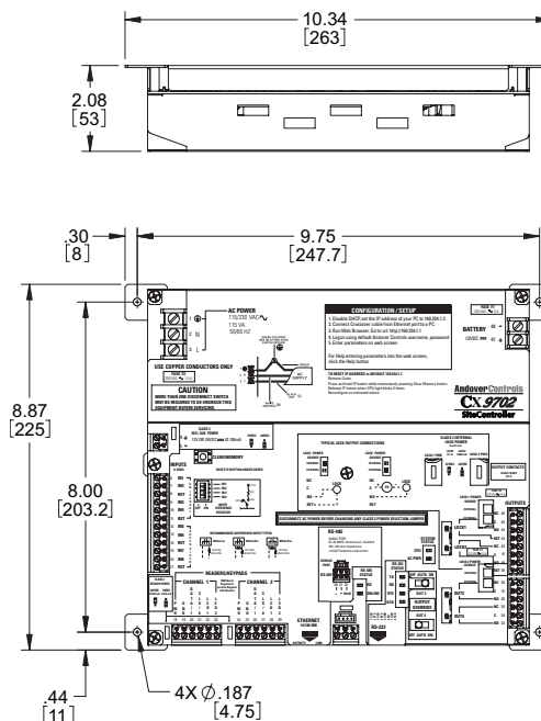
DIMENSIONAL DRAWINGS
